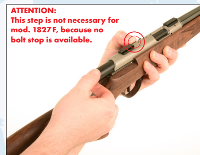
4. To remove the cleaning rod guide from the action, push and hold the bolt stop.
